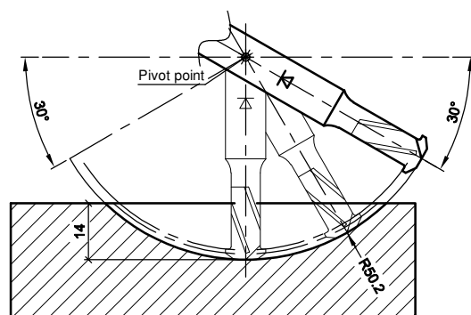
Shank cutter with 5 axis
