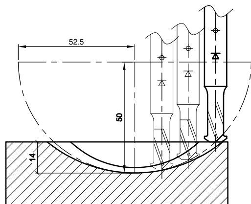
Shank cutter with 3 axis
